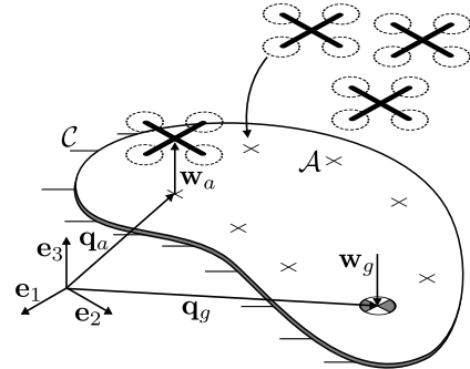
Fig. 1: A team of robots estimate the gravity wrench, \mathbf{w}_g , of a payload by iteratively selecting attachment points, \mathcal{A} , and applying wrenches, \mathbf{w}_a , that lead to reduction in COM location uncertainty while preserving system static equilibrium.
