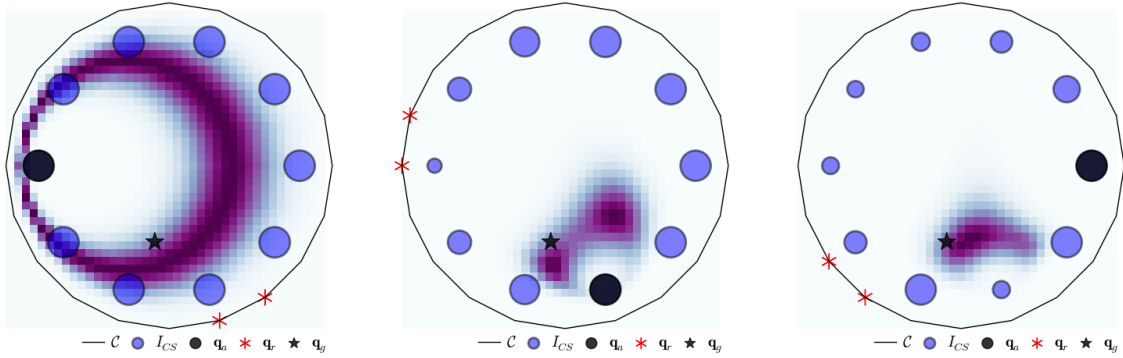
Fig. 2: Results of a simulated experiment with attachment points scaled by mutual information (blue) and the chosen attachment point (black) with active constraints, \mathbf{q}_r , denoted in red over the incrementally (left-to-right) updated belief distribution associated with the estimation of true COM location (black star).
